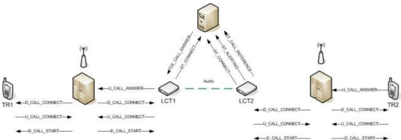
Downlink private call establishment (TR2 → TR1)
